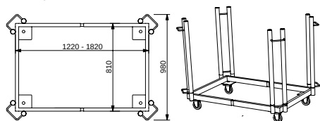
CARRELLO HIDE - HAND TRUK HIDE
